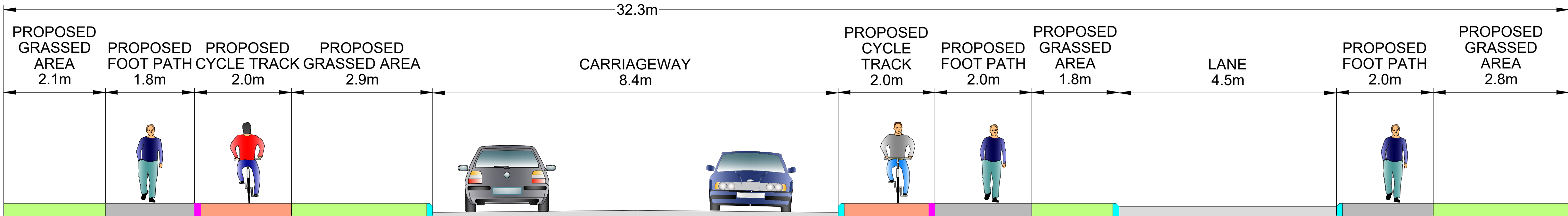
CROSS SECTION Q-Q
